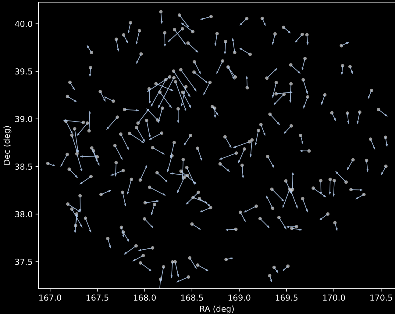
APOGEE DR17 Cluster 1 Proper Motion Vectors (n=185)
