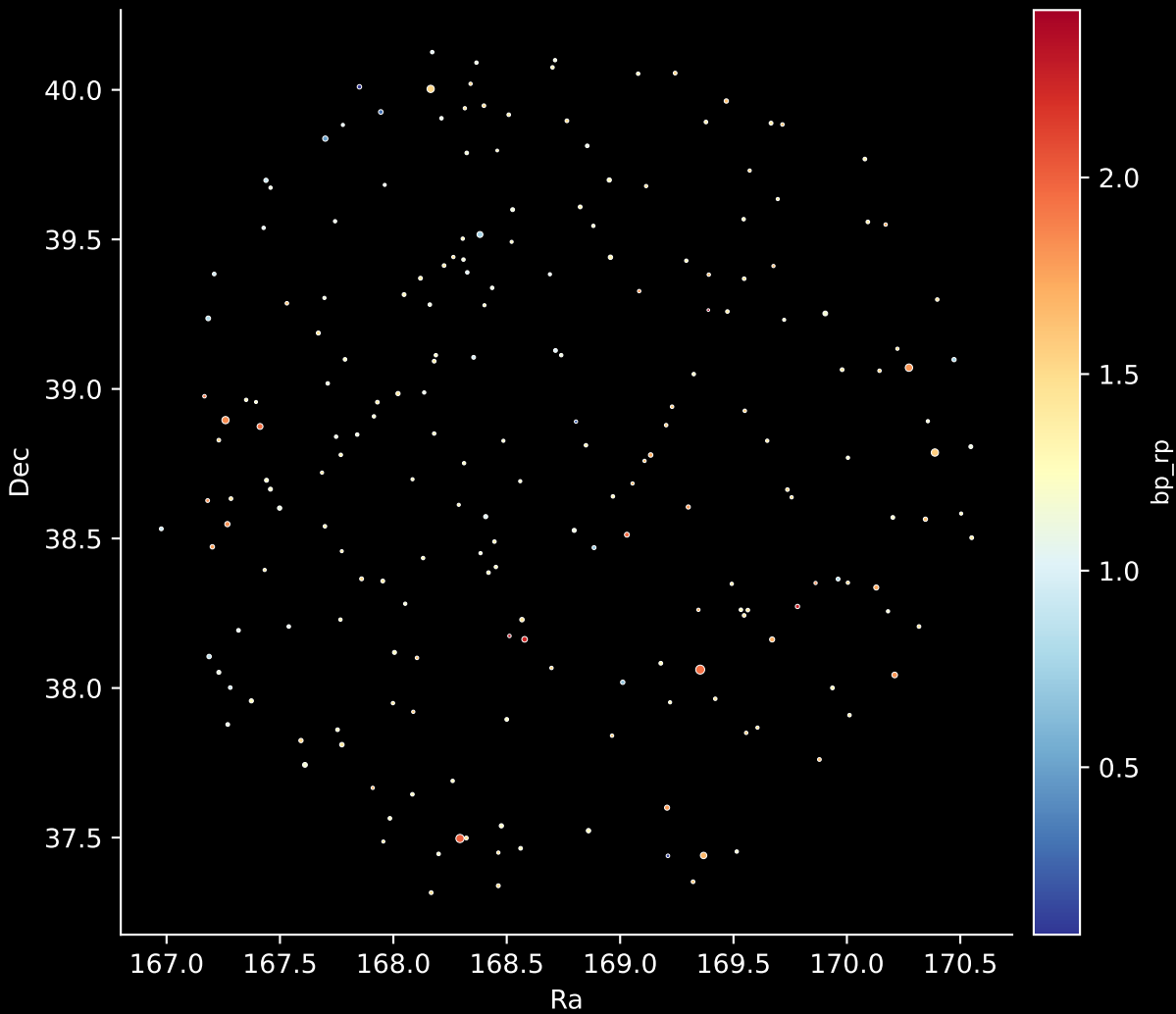
APOGEE DR17 Field: [CA_163-05_btx] Stars: 211
