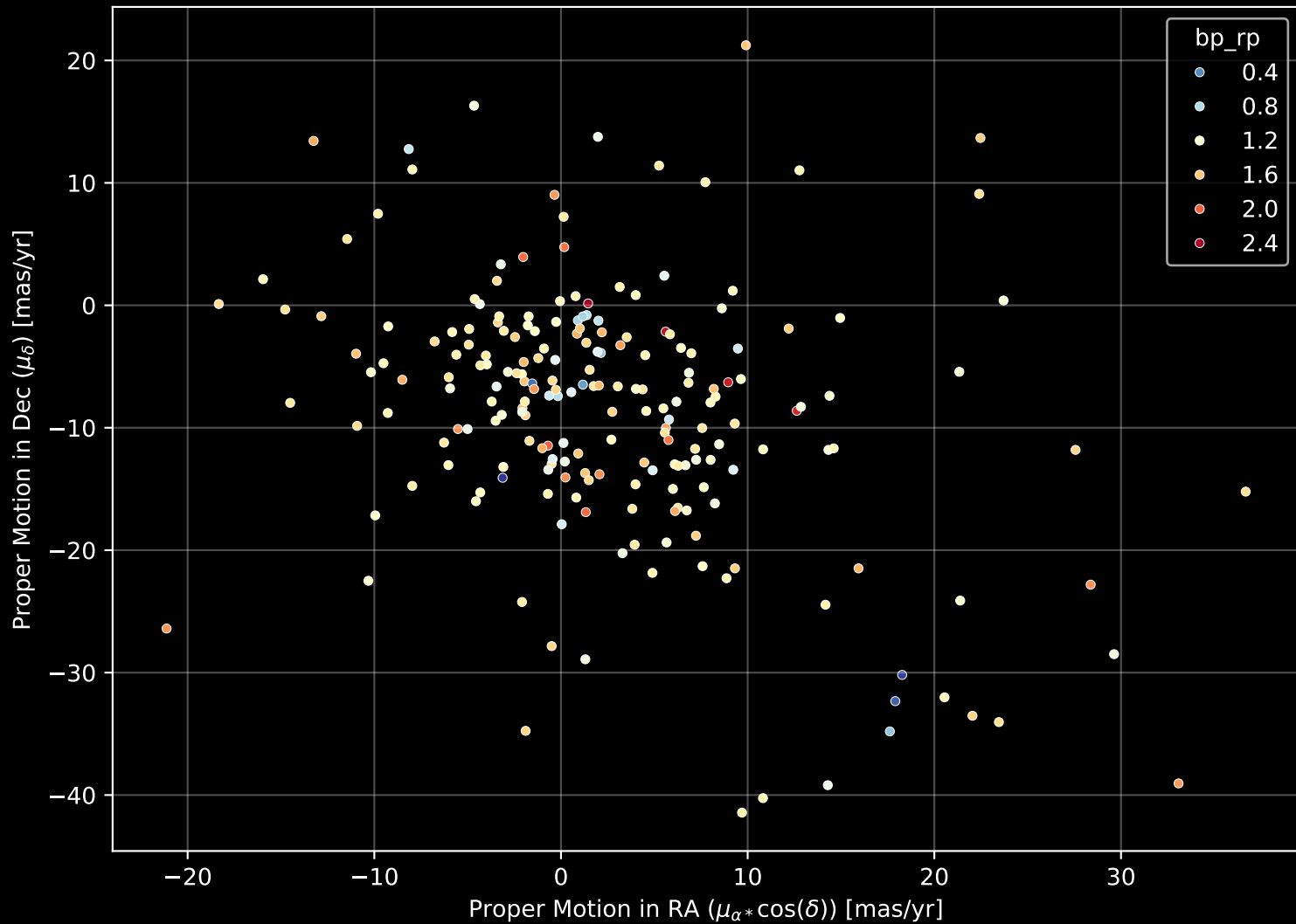
APOGEE DR17 Field: [CA_163-05_btx] Proper Motion Diagram (n= 211)
