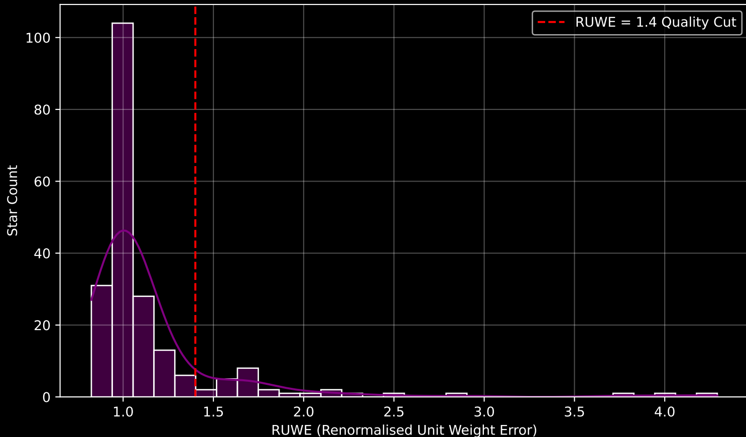
GAPOGEE DR17 Field [CA_163-05_btx] RUWE Distribution (n= 209)
