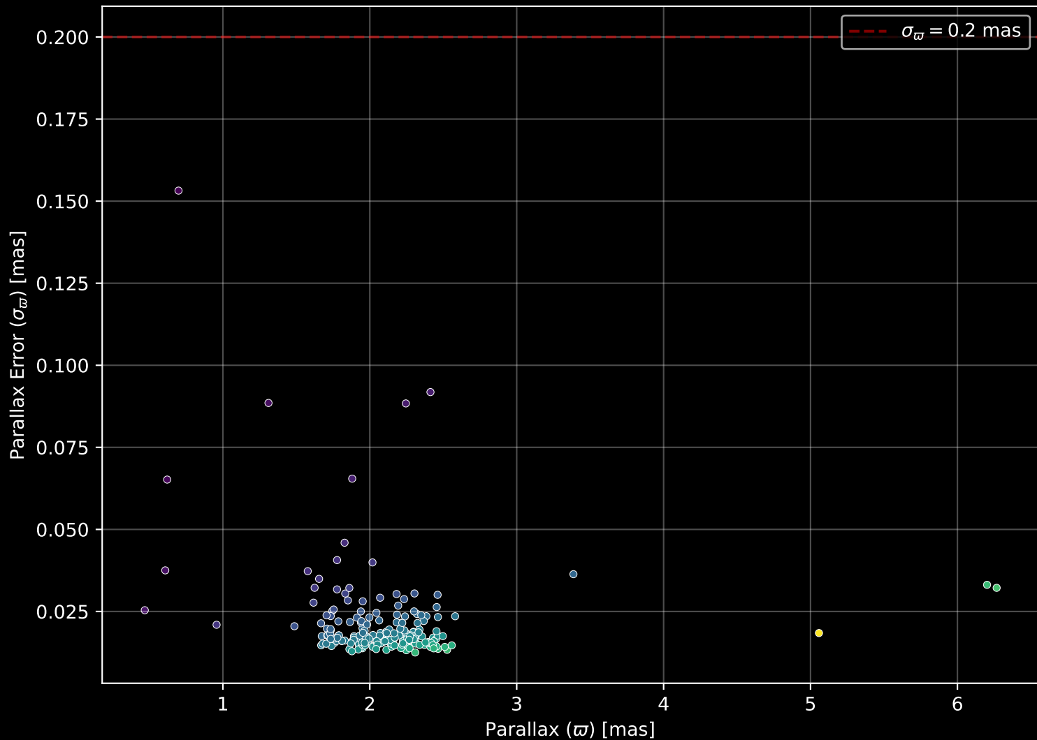
APOGEE DR17 Field: [CA_163-05_btx] Parallax Quality (n= 211)
