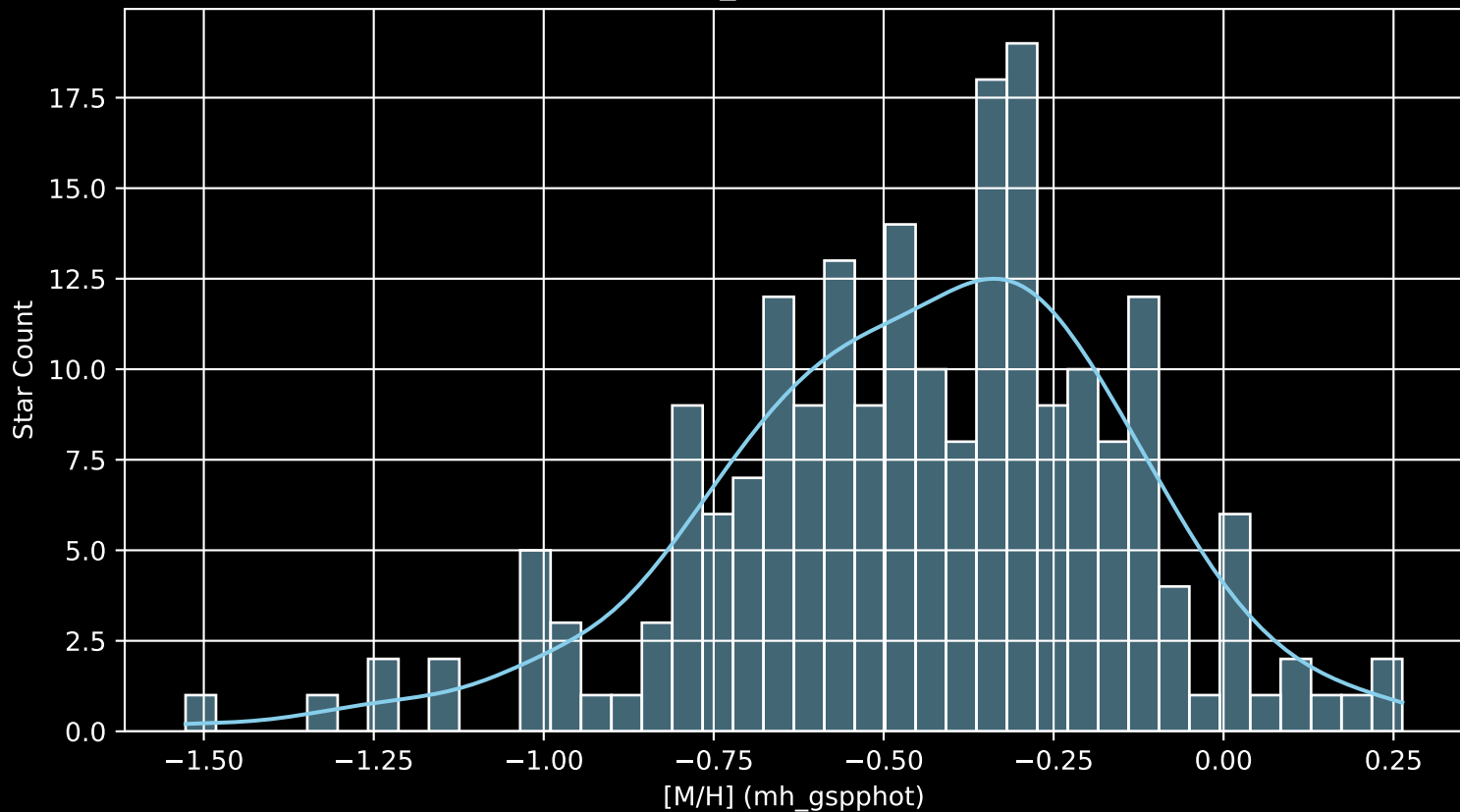
APOGEE DR17 Field: [CA_163-05_bt [M/H] (mh_gspphot) (n= 210)
