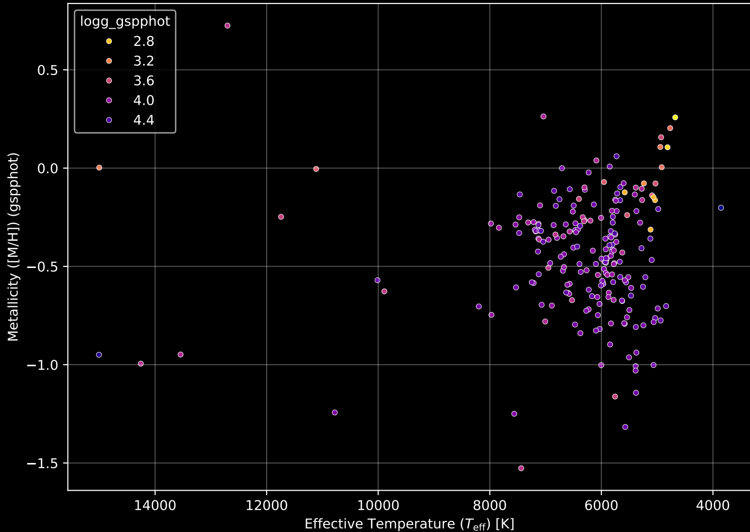
APOGEE DR17 Field: [CA_163-05_btx] Stellar Population Parameters (n= 211)
