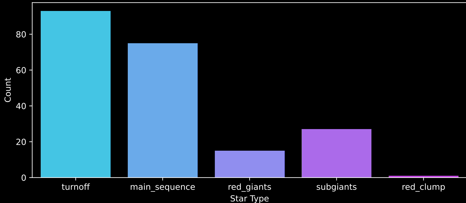
APOGEE DR17 Field: [CA_163-05_btx] Count plot of Star Type
